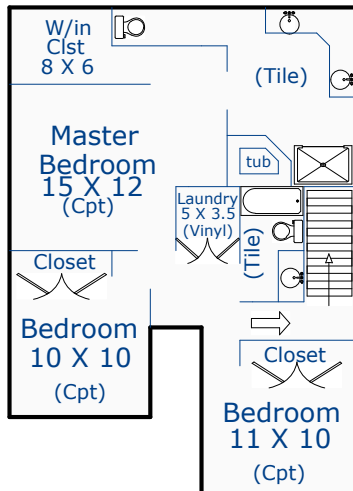
Second Floor 908 sf
